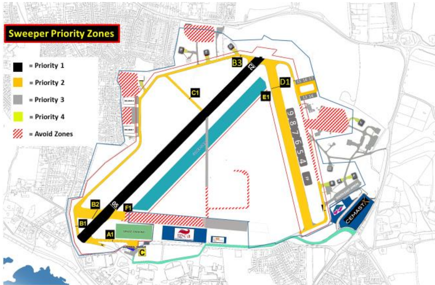
Figure 3 - Sweeper Plan
